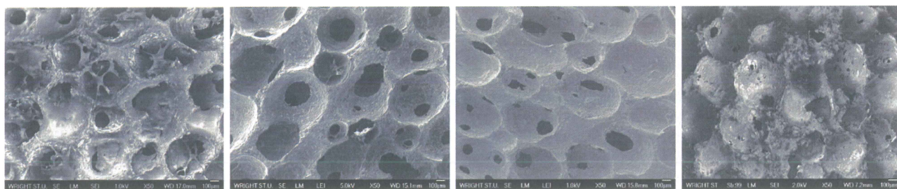
Fig. 2. SEM images of Uncoated foam (UC), Silicon Dioxide ( \text{SiO}_2 ) coated foam, Collagen Coated (CC) foam, and Carbon Nanotube (CNT) Coated foam shown respectively. Pictures are of the cells grown on each of the coated foams for 72 hours.
